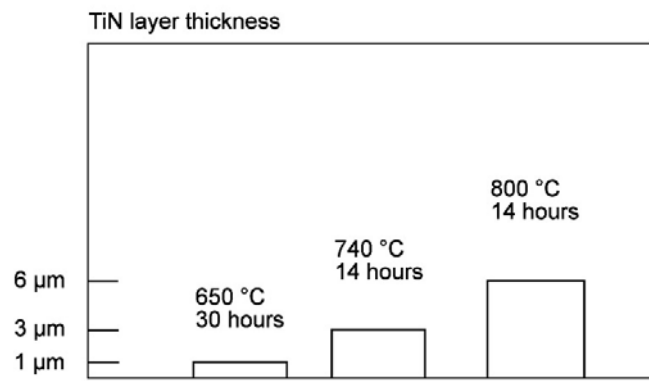
Figure 3: Time and temperature dependence on the TiN - layer thickness.
