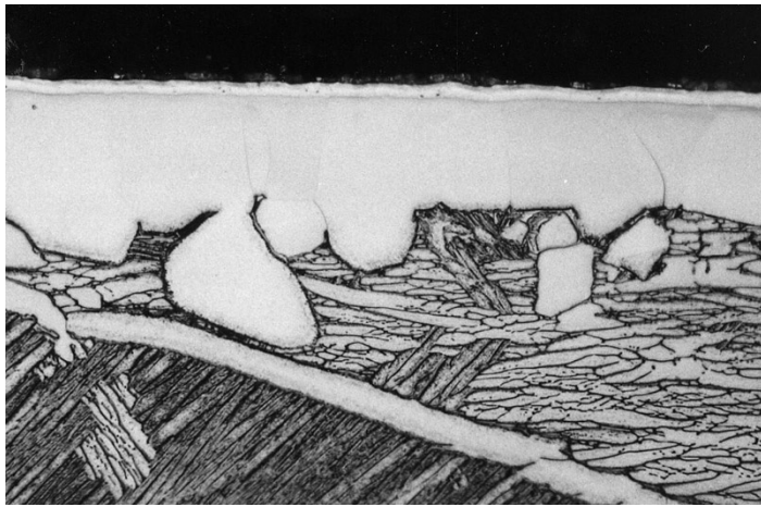
Figure 4: Nitrided structure, etched in 2% HF (IWT Bremen).
